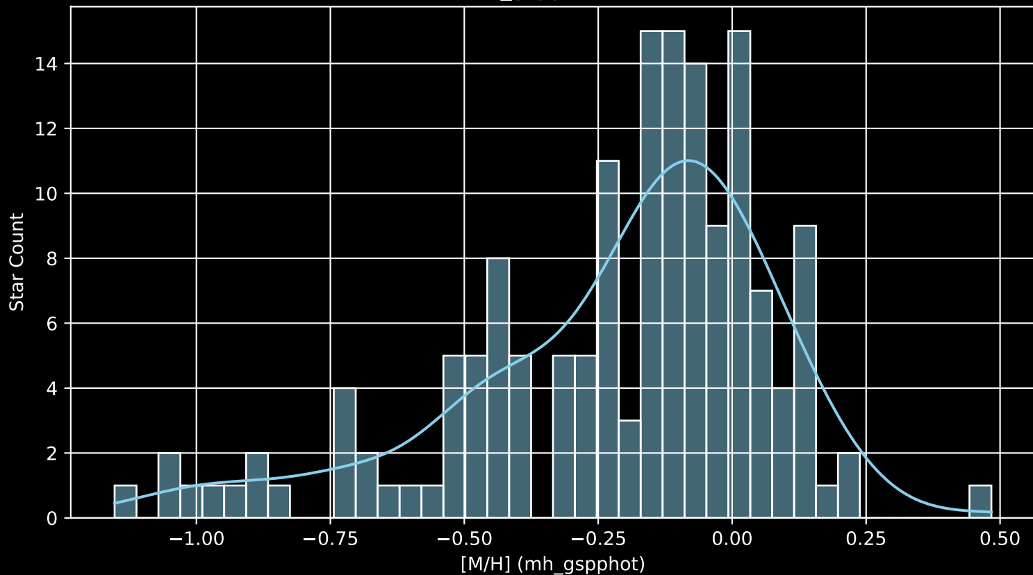
APOGEE DR17 Field: [235+06 [M/H] (mh_gspphot) (n= 157)
