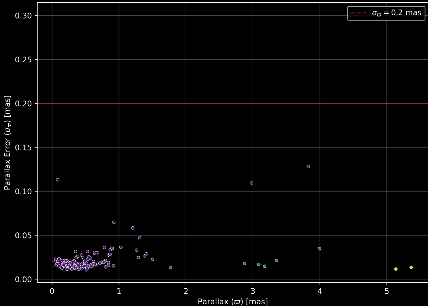
APOGEE DR17 Field: [235+06] Parallax Quality (n= 159)
