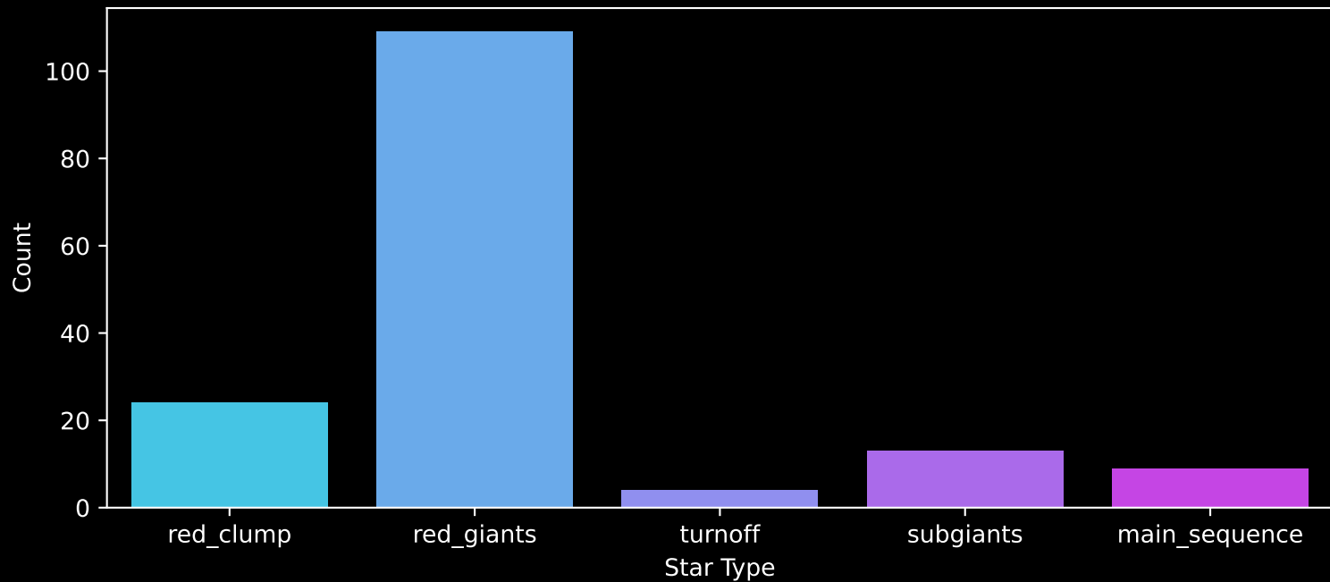
APOGEE DR17 Field: [235+06] Count plot of Star Type
