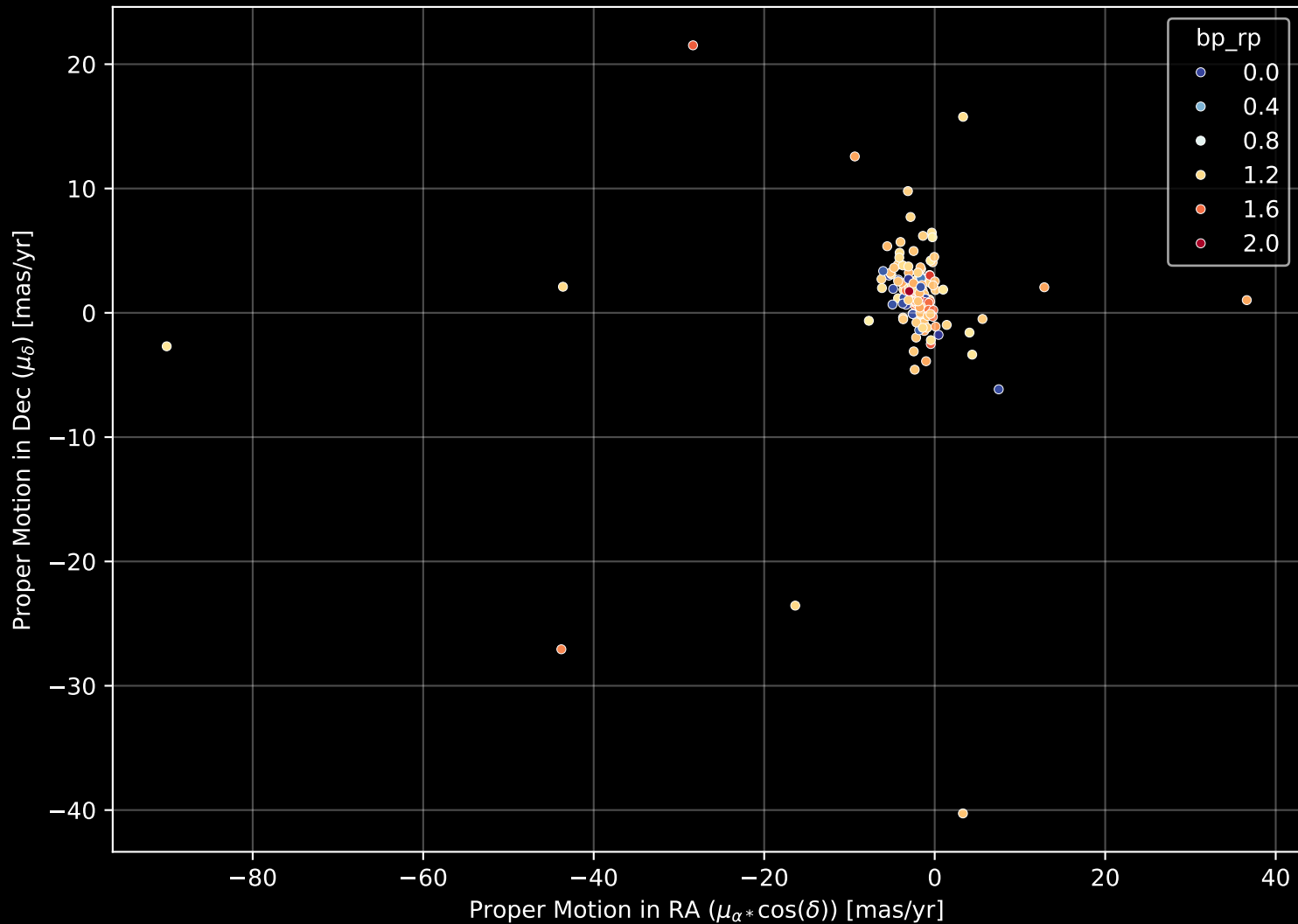
APOGEE DR17 Field: [235+06] Proper Motion Diagram (n= 159)
