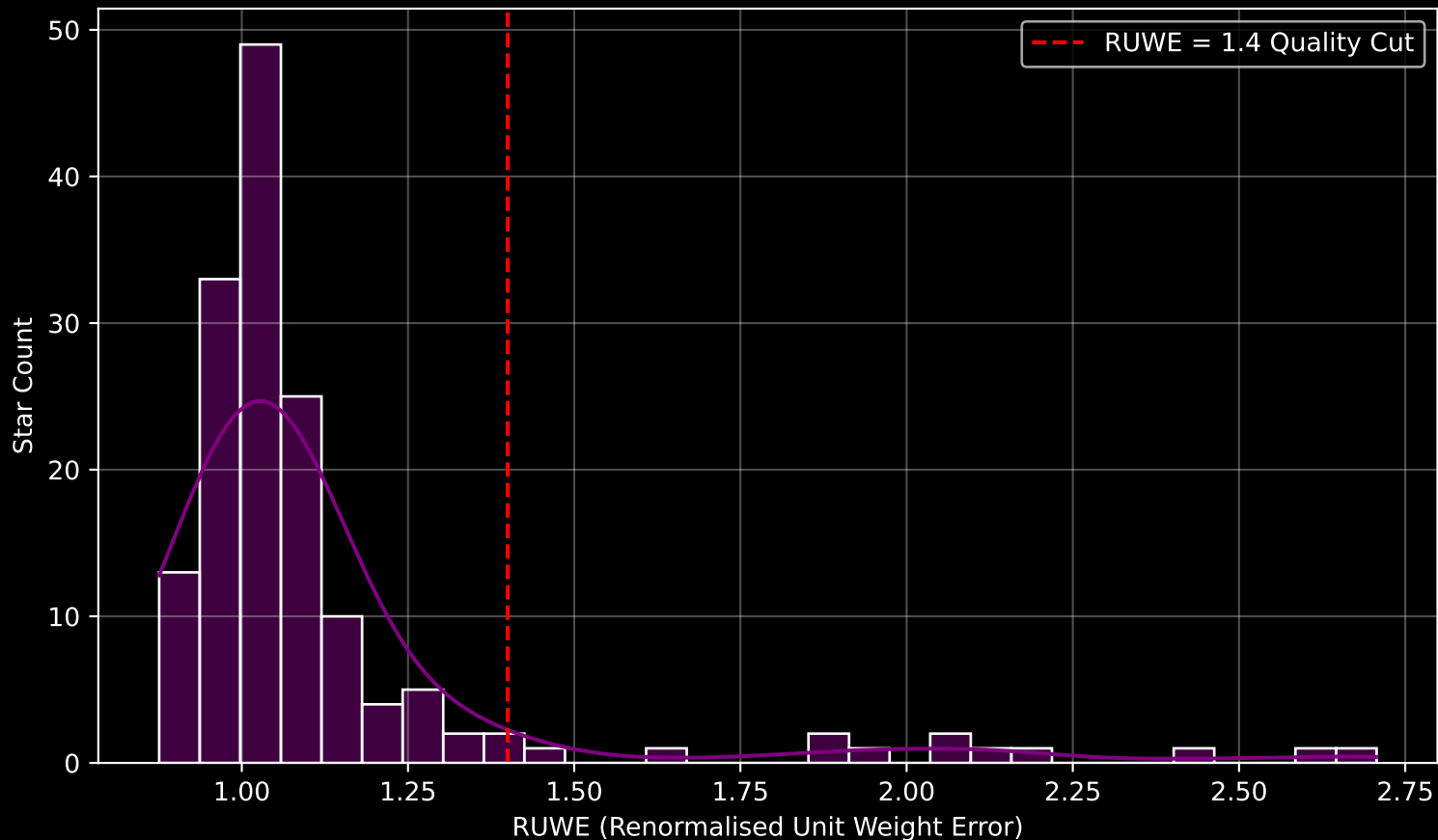
GAPOGEE DR17 Field [235+06] RUWE Distribution (n= 155)
