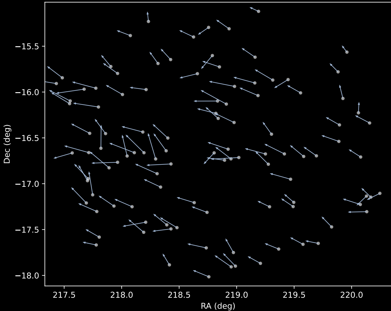
APOGEE DR17 Cluster 1 Proper Motion Vectors (n=106)
